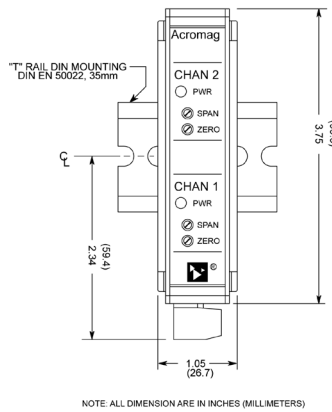
650T ISOLATOR ENCLOSURE DIMENSIONS
