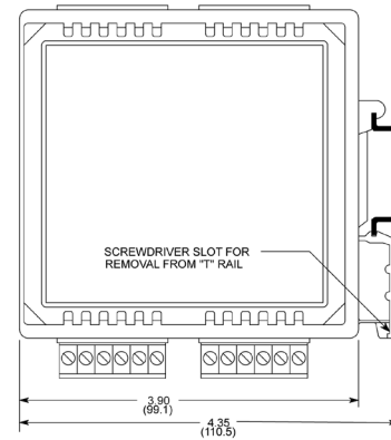
650T ISOLATOR ENCLOSURE DIMENSIONS
